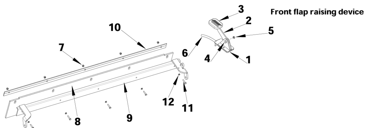
Accelerator pedal assembly
