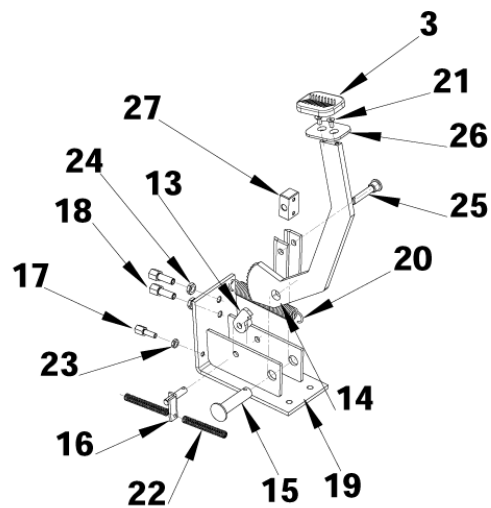
Brake pedal assembly
